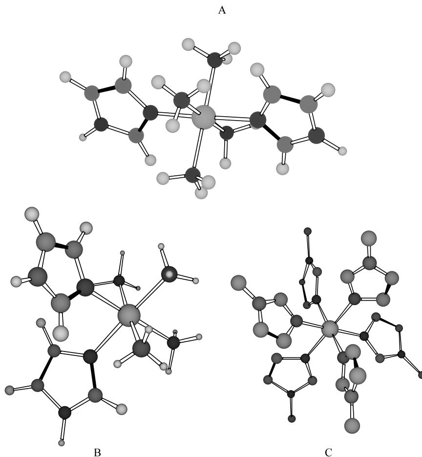
Fig. 13. Structures of ruthenium immunosuppressant complexes: (A) trans -[(Im) 2 (NH 3 ) 4 Ru] 3+ [356], (B) cis -[(Im) 2 (NH 3 ) 4 Ru] 2+ , (C) [(1MeIm) 6 -Ru] 2+ [324]. Hydrogen atoms omitted from C for clarity.
