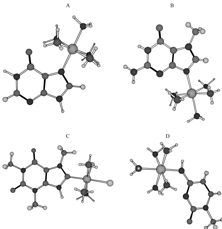
Fig. 2. Structures of a) [(\text{Hyp}\kappa^7)(\text{NH}_3)_5\text{Ru}]^{3+} showing the typical N7 coordination of many transition metal ions at the N7 of a purine [101]; b) [(7\text{MeGuak}^7)(\text{NH}_3)_5\text{Ru}]^{3+} , depicting one of the linkage isomers present when N9 is also available for bonding [36]; c) cis - [\text{Cl}_2(1,3,7\text{Me}_3\text{Xan}\kappa^8)-(\text{NH}_3)_3\text{Ru}]^{3+} illustrating an unusual carbon-bound form of caffeine bound to ruthenium; and d) [(1\text{MeCyt}\kappa^{\text{N}4})\text{Cl}(\text{NH}_3)\text{Ru}]^{2+} portraying binding to an ionized exocyclic amine.
